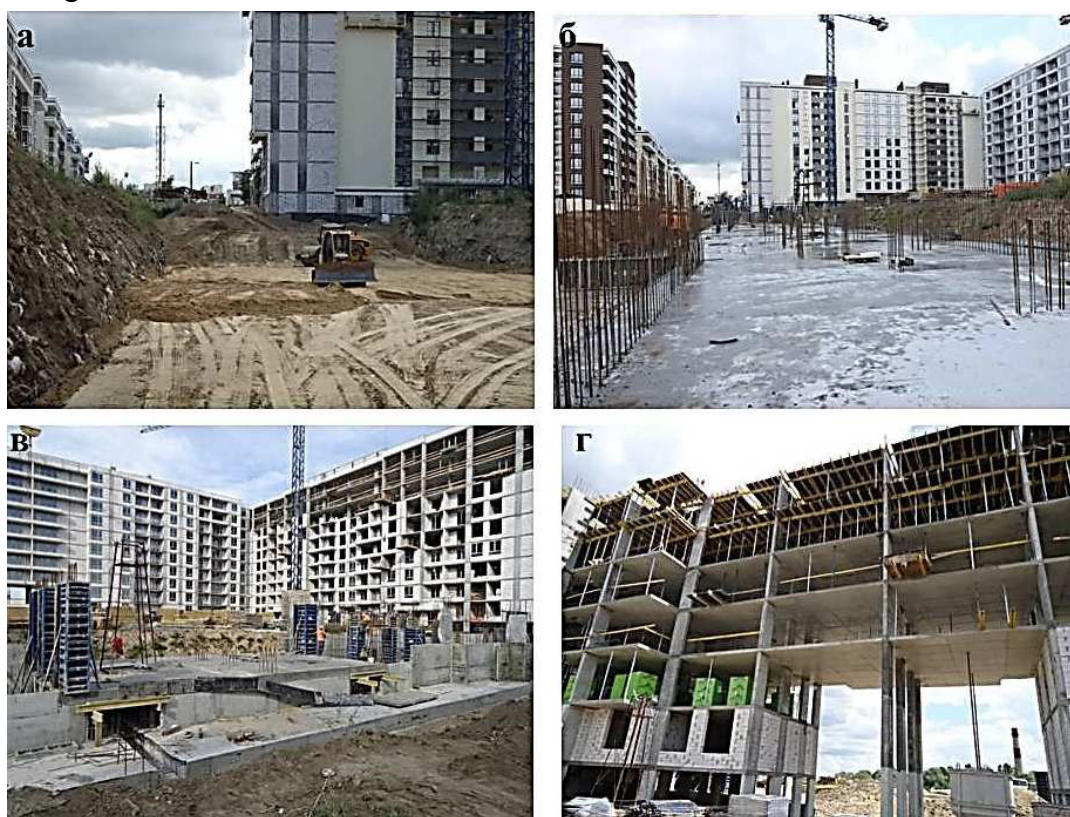
Fig. 6. General view performance of work: preparation of foundation (a); the device of the foundation slab (b); the device of basement (c); building frame (d)
