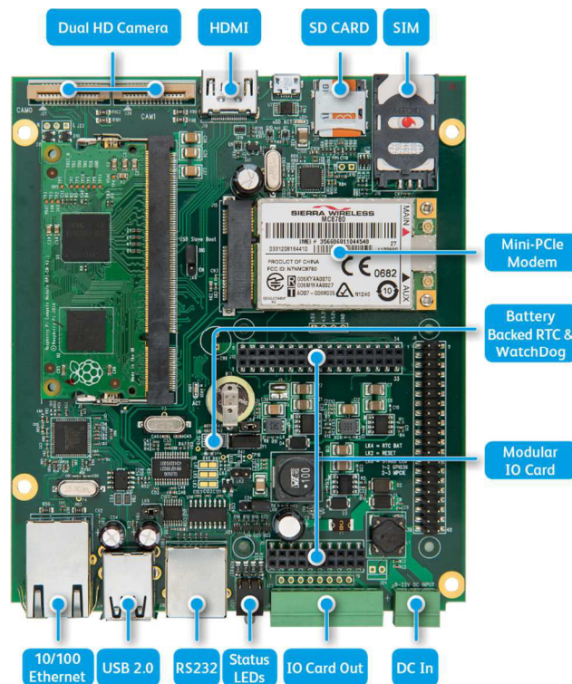
Fig. 4. Industrial IoT Integrator Board (MyPi) [6]
