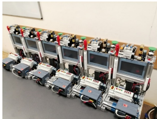
Fig. 11. Fully equipped training stands with programmable logic controllers
