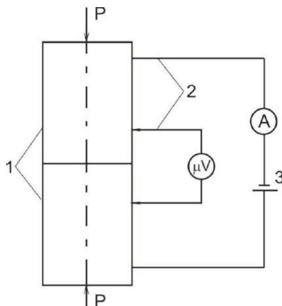
Fig. 9. The Scheme of electrical resistance measurement in the welding zone using the four-probe method:
